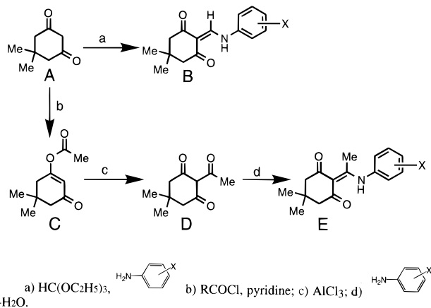
Figure 1. General synthetic route for phenylaminoalkylidene-1,3-cyclohexanedione analogues.
